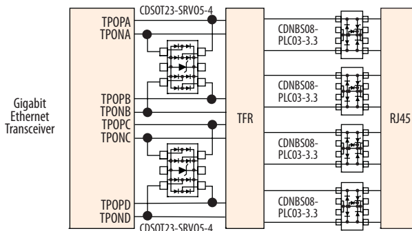
Gigabit Ethernet (GR 1089) Intra-Building Protection
